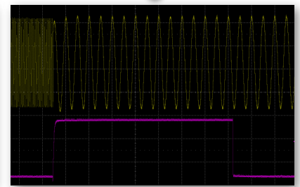
Sweep-Frequency Start Sync 15 \mu s Pulse
