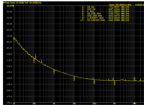
Phase Noise Performance (REFCLK: 1 GHz TCXO) -139 dBc/Hz, 20 kHz Offset 397.8 MHz +10 dBm
