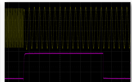
Sweep-Frequency Start Sync 15 \mu s Pulse EXT Free Run (Trigger Out)
